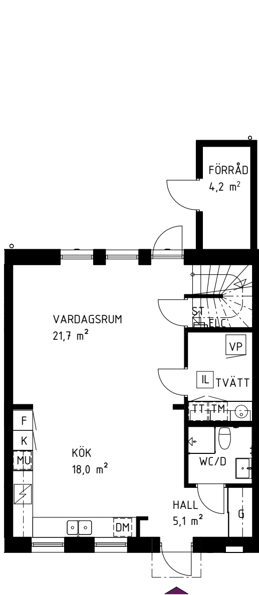
BOTTENPLAN
