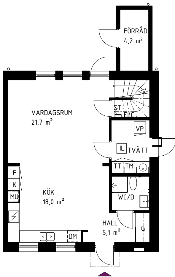
BOTTENPLAN
