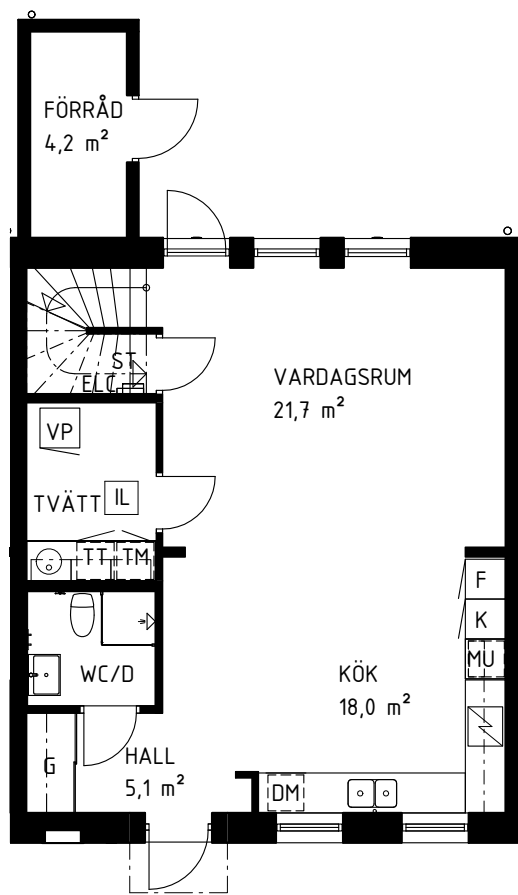
BOTTENPLAN
