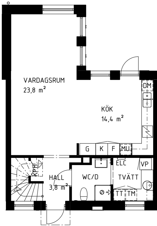
BOTTENPLAN
