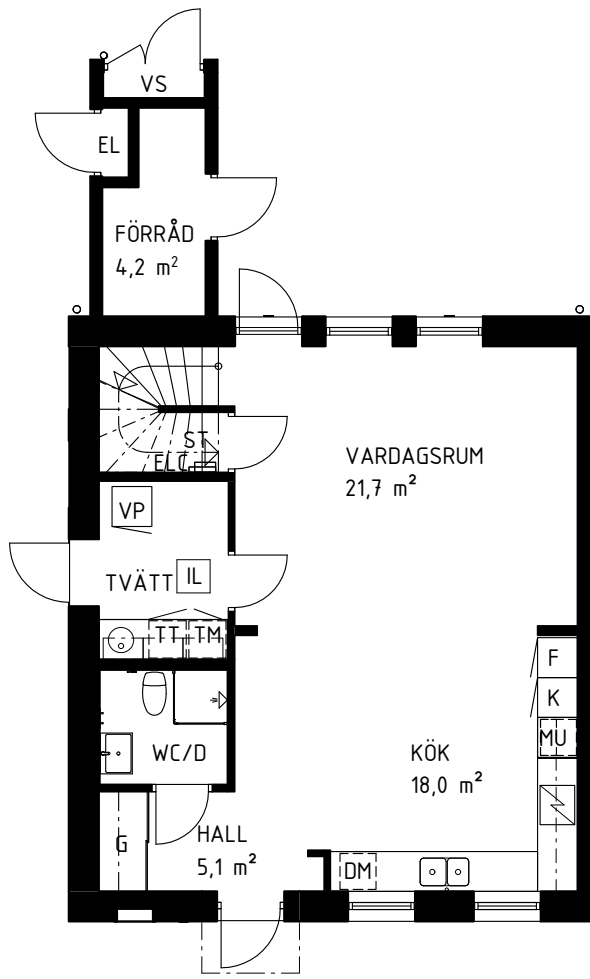
BOTTENPLAN
