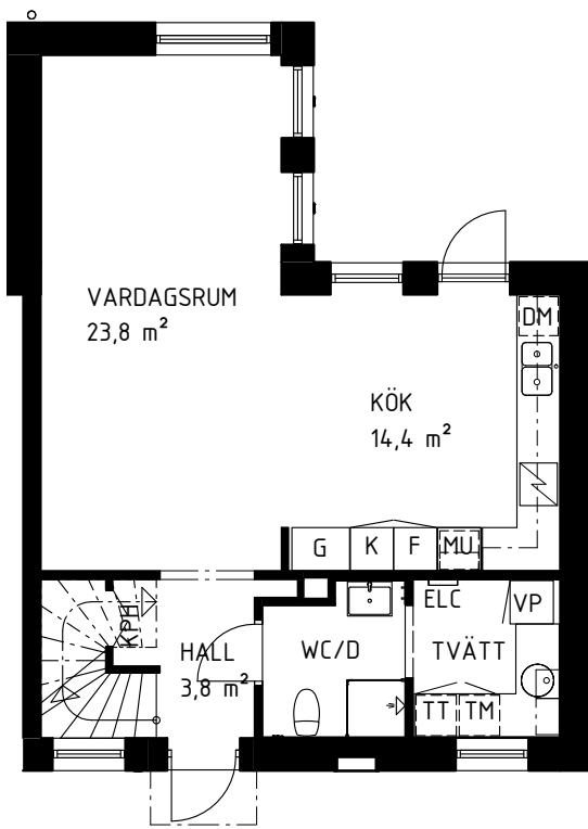
BOTTENPLAN
